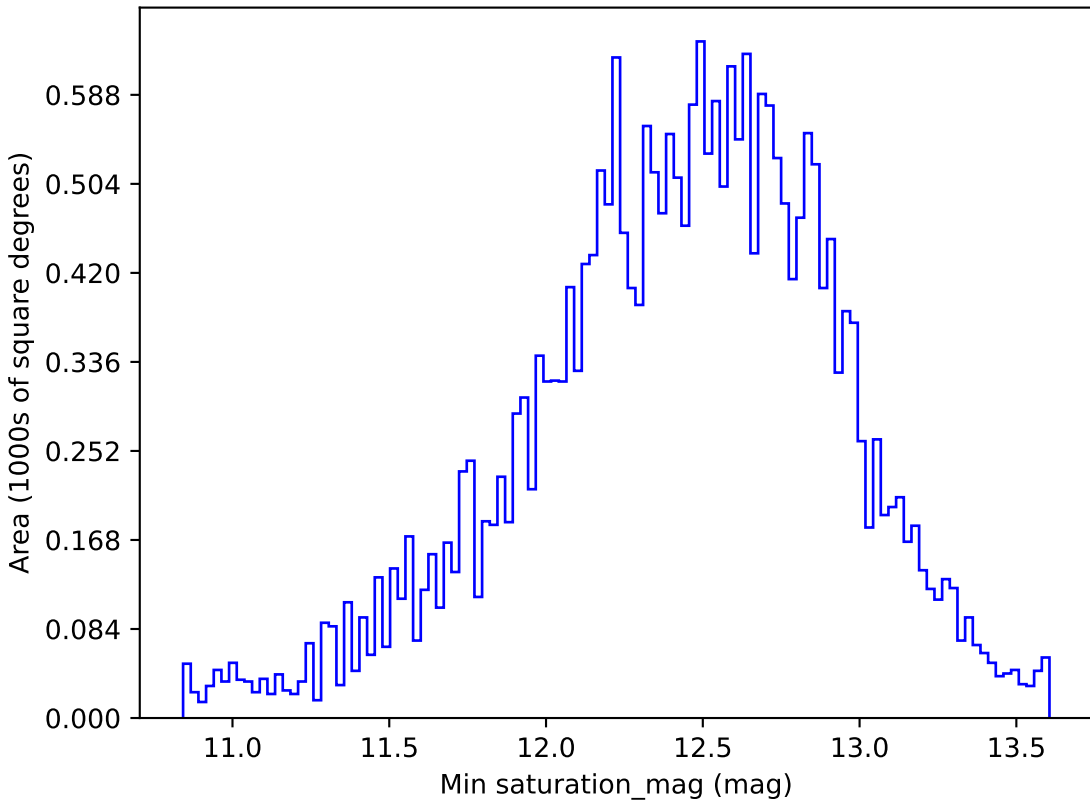
too_5_1v3.4_10yrs All sky i band: Min saturation_mag
