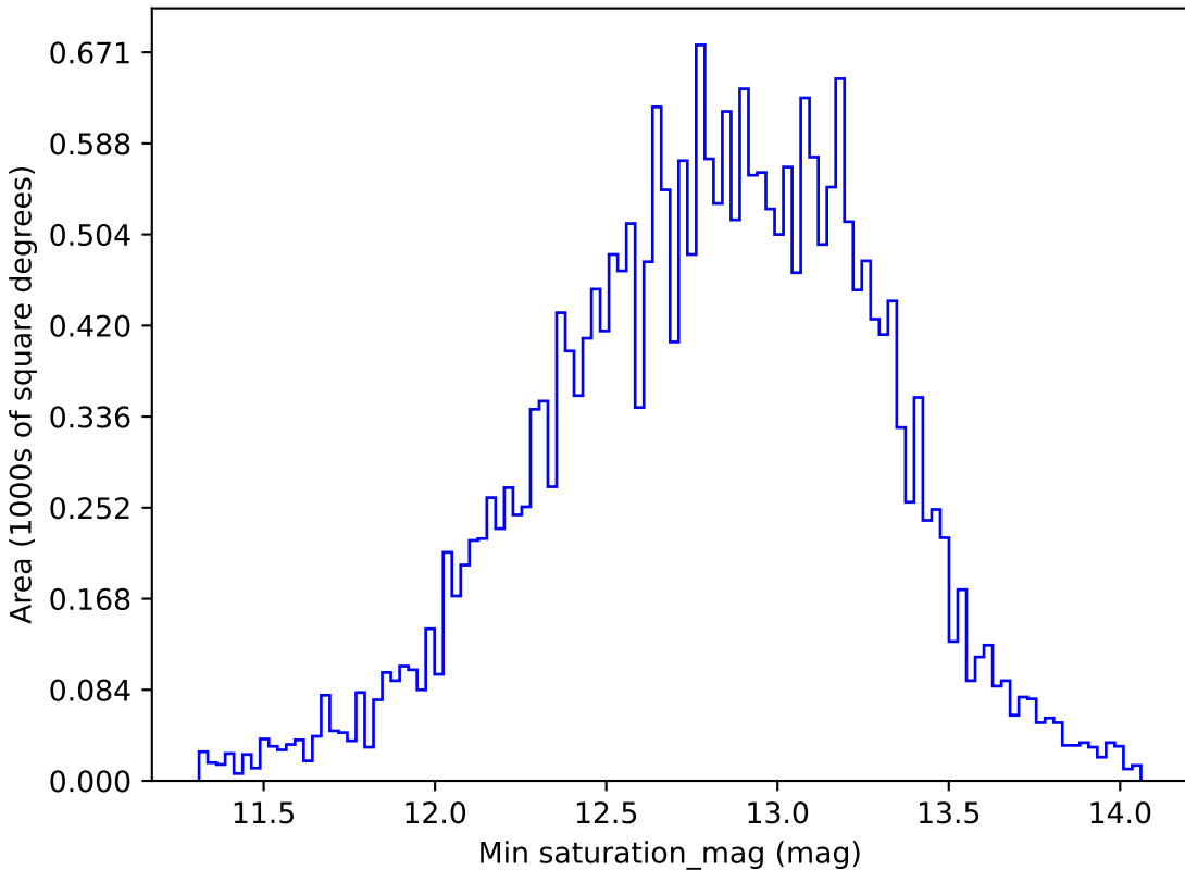
too_5_1v3.4_10yrs All sky g band: Min saturation_mag
