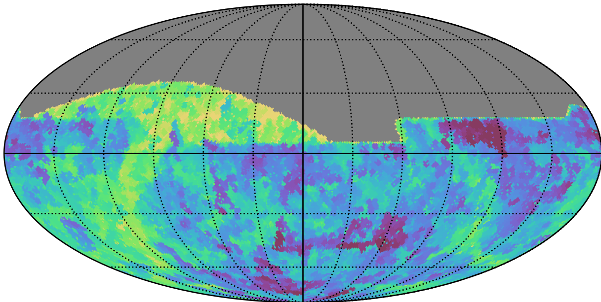
too_5_1v3.4_10yrs All sky all bands: Min saturation_mag
