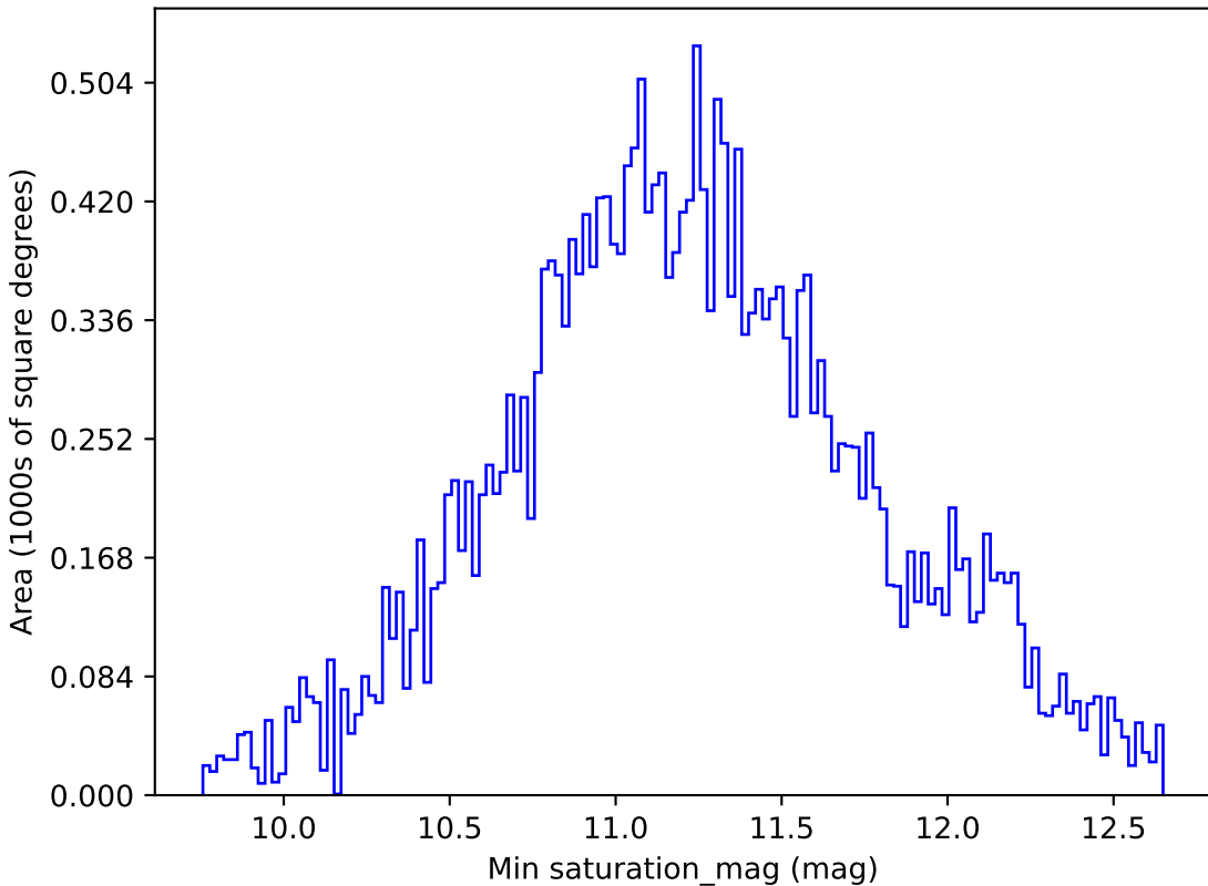
too_5_1v3.4_10yrs All sky all bands: Min saturation_mag
