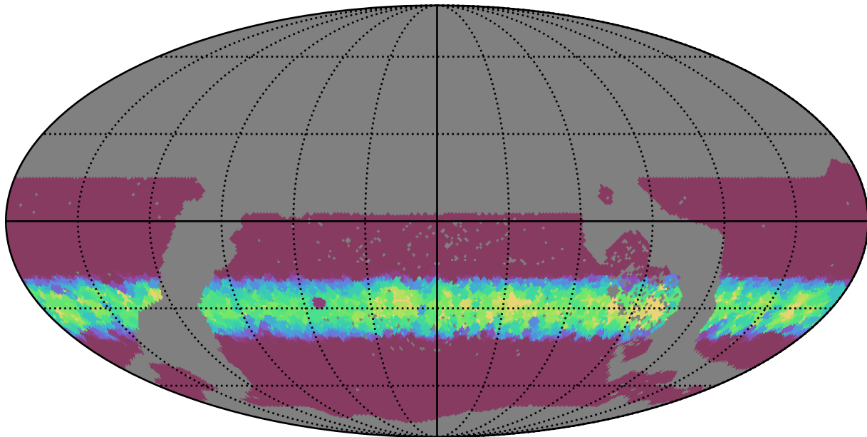
too_5_1v3.4_10yrs WFD z band: Min normairmass
