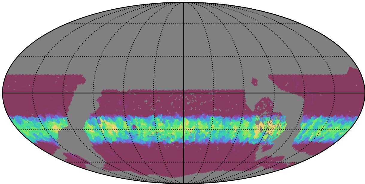
too_5_1v3.4_10yrs WFD u band: Min normairmass
