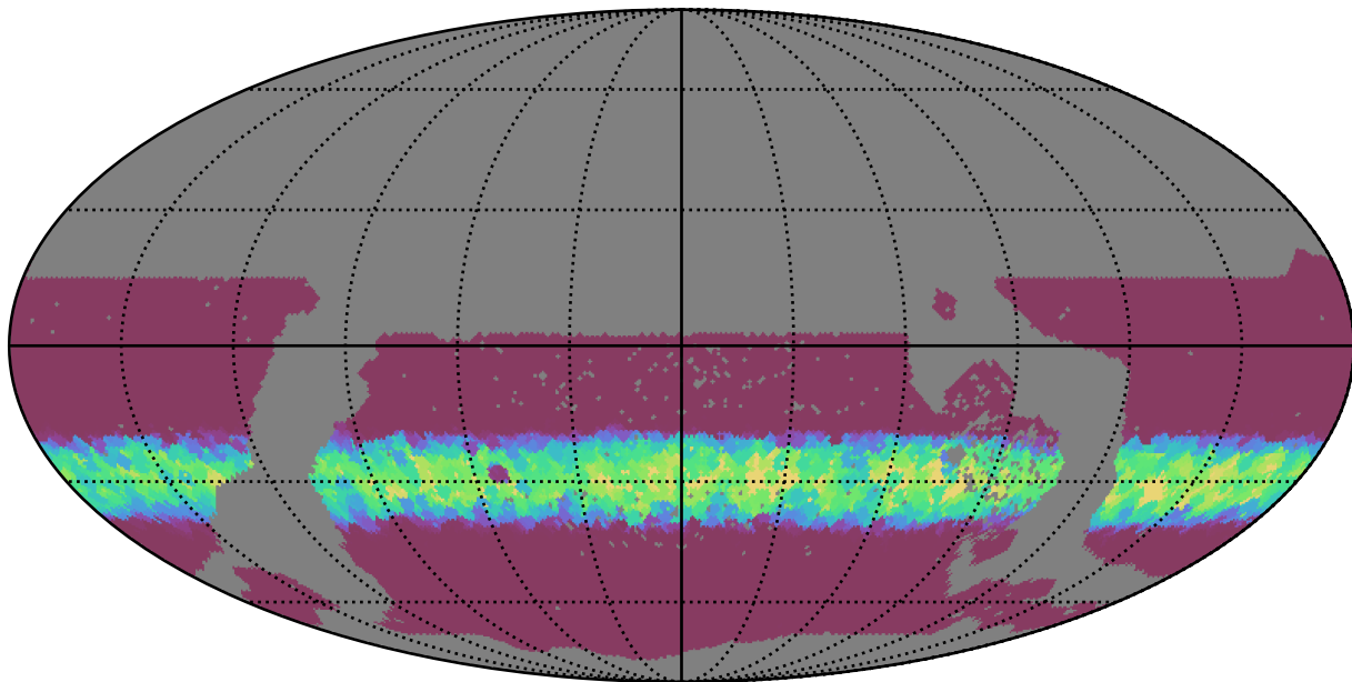
too_5_1v3.4_10yrs WFD r band: Min normairmass
