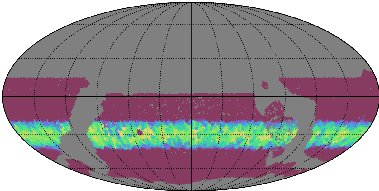
too_5_1v3.4_10yrs WFD g band: Min normairmass
