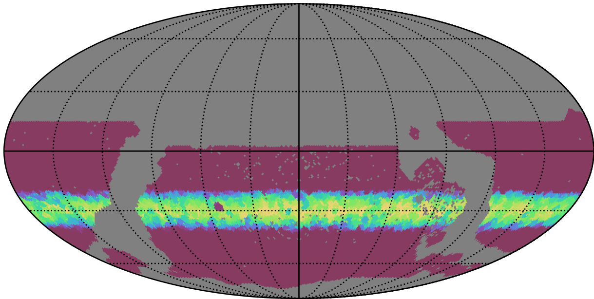
too_5_1v3.4_10yrs WFD all bands: Min normairmass
