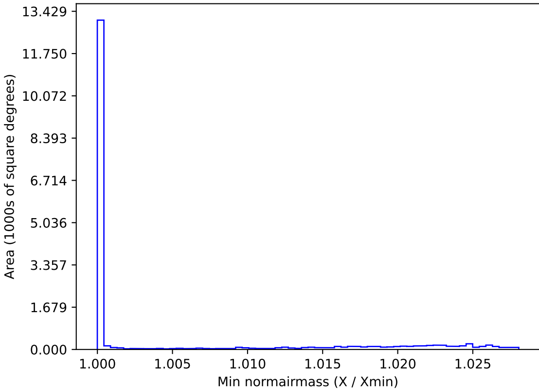
too_5_1v3.4_10yrs WFD all bands: Min normairmass
