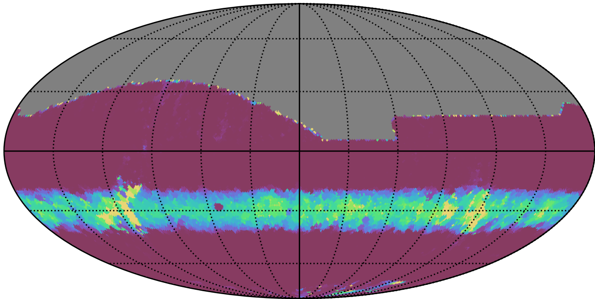
too_5_1v3.4_10yrs All sky z band: Min normairmass
