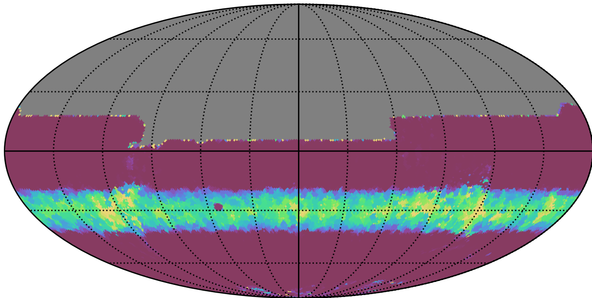
too_5_1v3.4_10yrs All sky y band: Min normairmass
