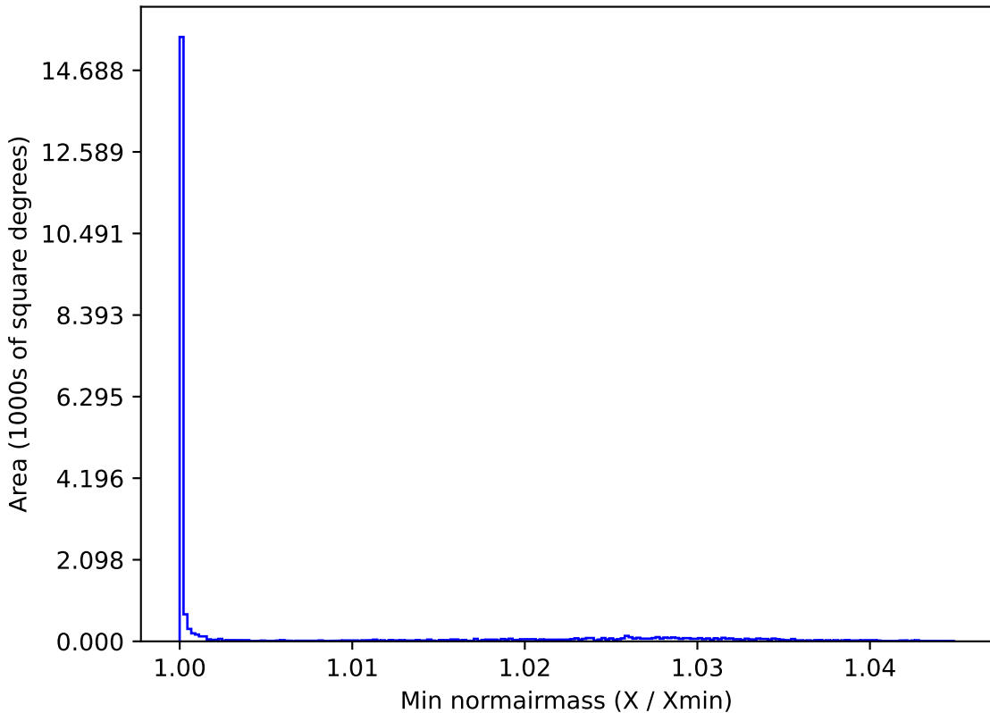
too_5_1v3.4_10yrs All sky y band: Min normairmass
