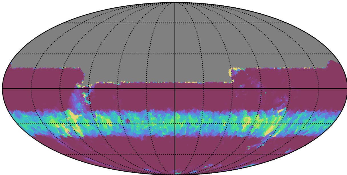
too_5_1v3.4_10yrs All sky u band: Min normairmass
