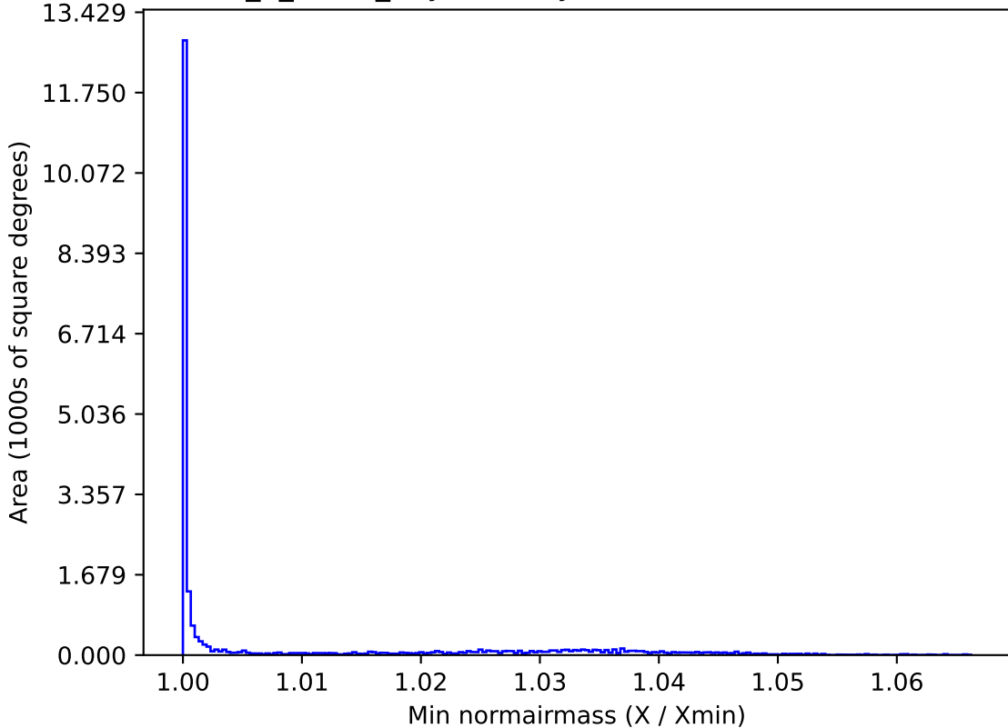
too_5_1v3.4_10yrs All sky u band: Min normairmass
