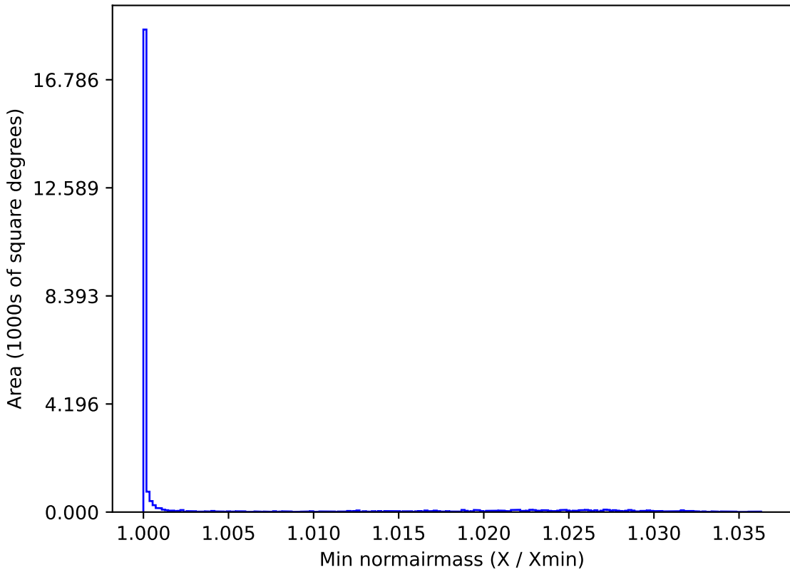
too_5_1v3.4_10yrs All sky r band: Min normairmass
