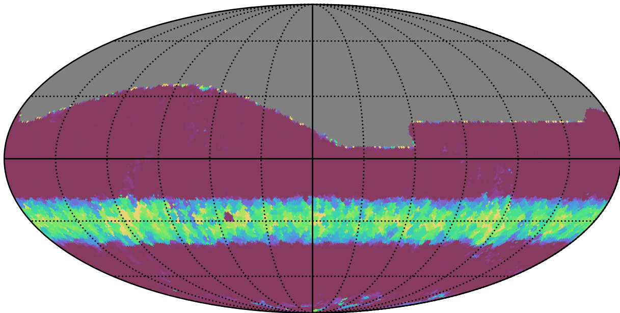
too_5_1v3.4_10yrs All sky g band: Min normairmass
