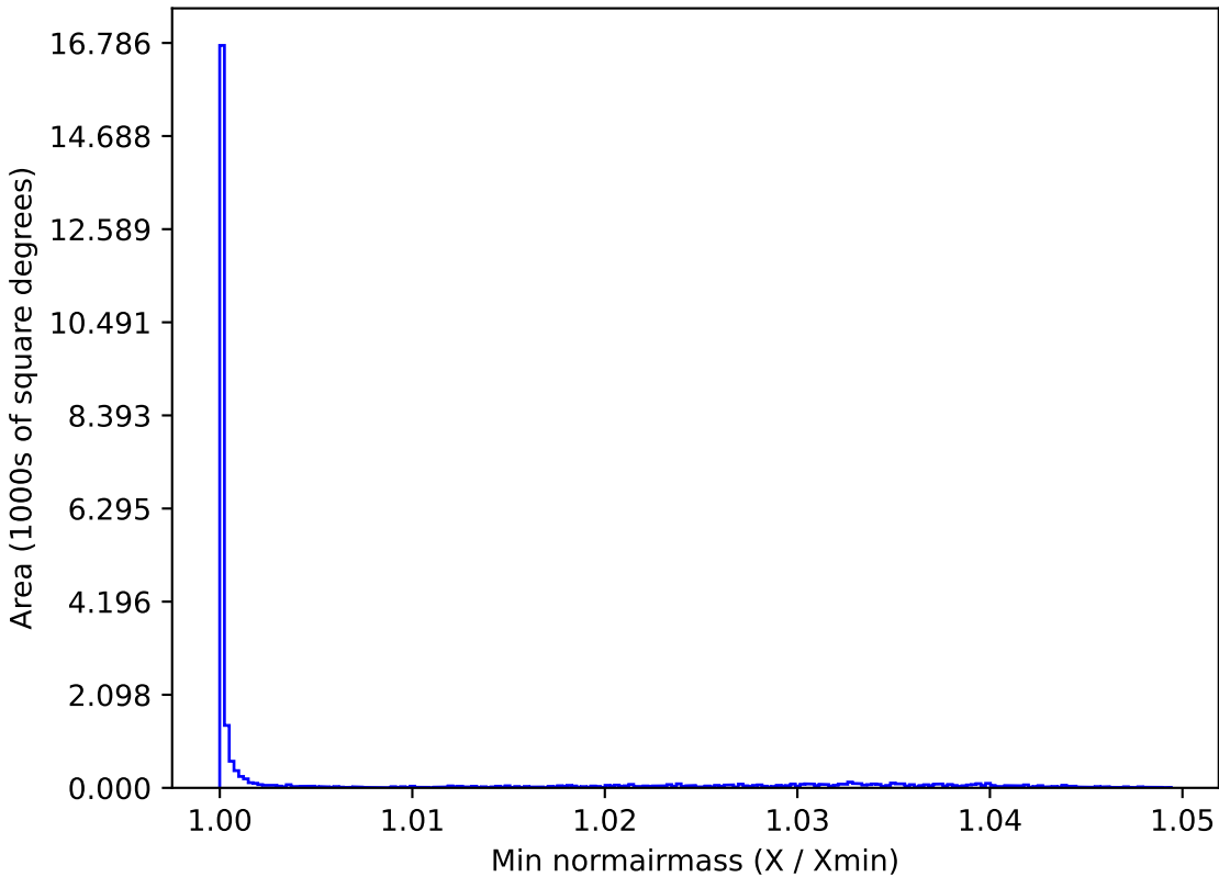
too_5_1v3.4_10yrs All sky g band: Min normairmass
