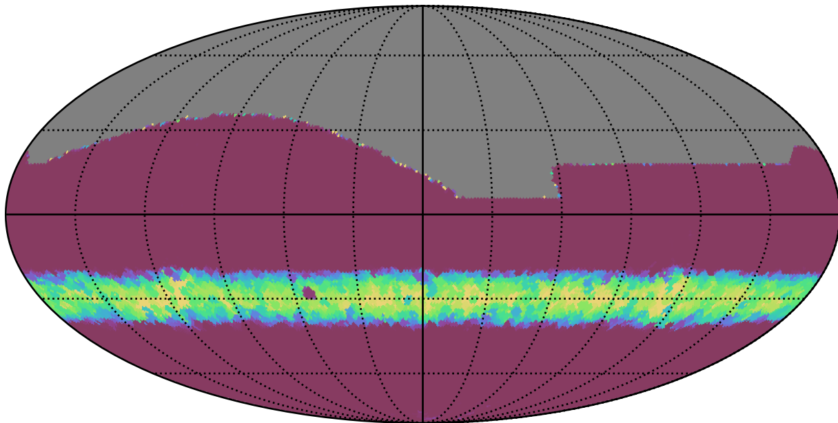
too_5_1v3.4_10yrs All sky all bands: Min normairmass
