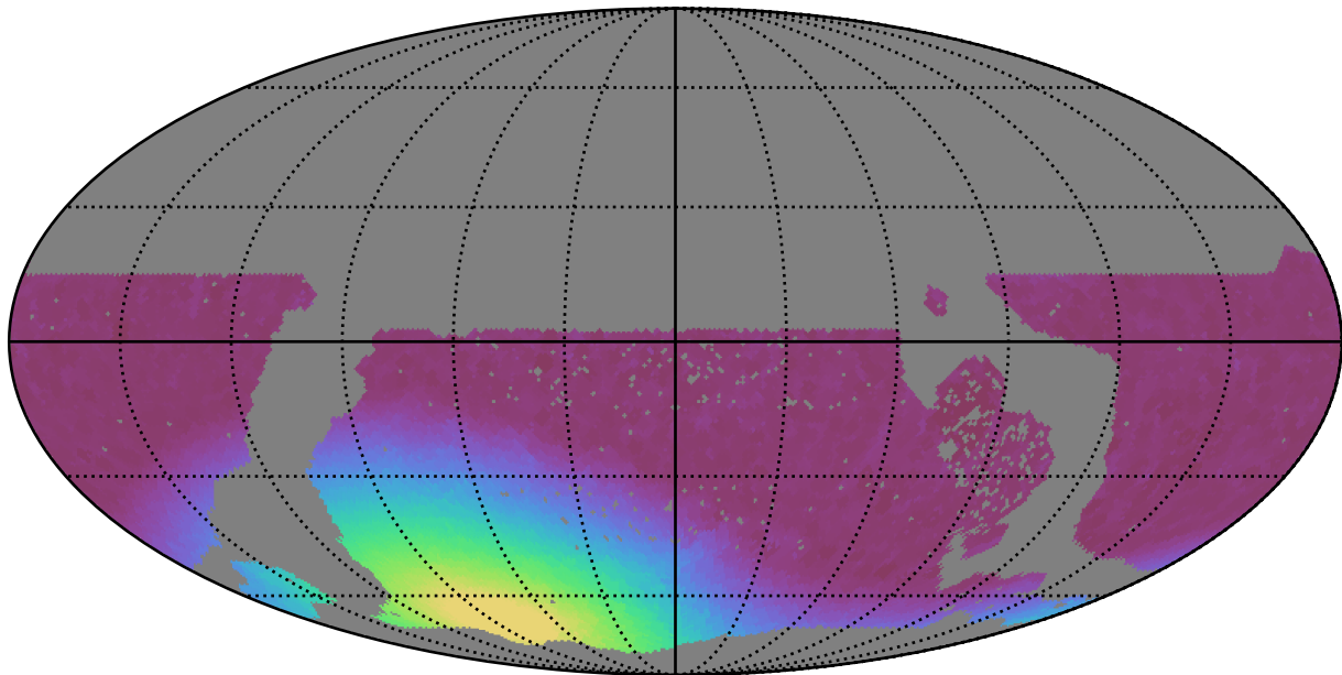
too_5_1v3.4_10yrs WFD z band: Min moonDistance
