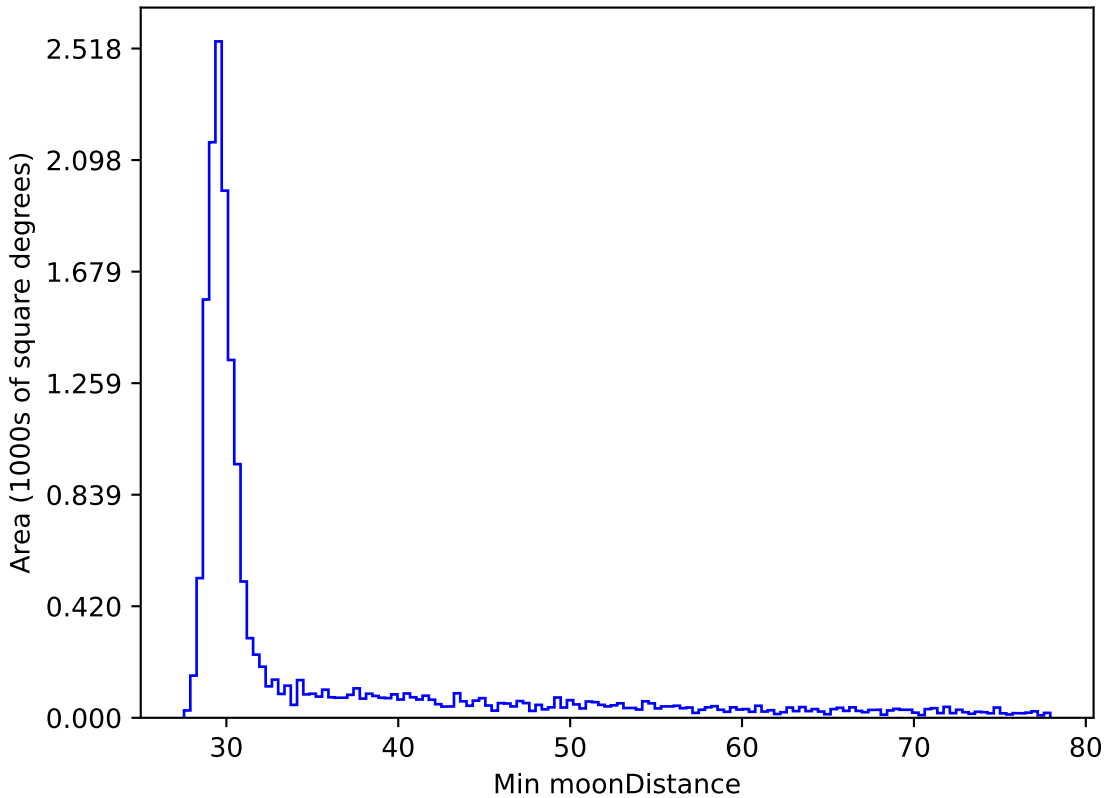
too_5_1v3.4_10yrs WFD z band: Min moonDistance
