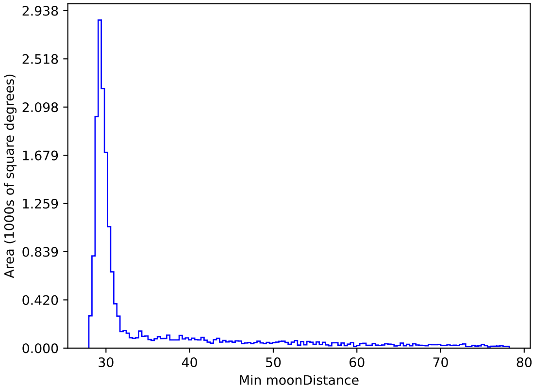
too_5_1v3.4_10yrs WFD y band: Min moonDistance
