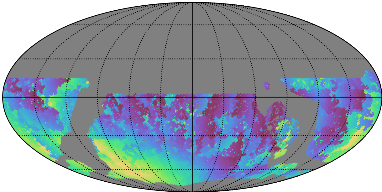
too_5_1v3.4_10yrs WFD u band: Min moonDistance
