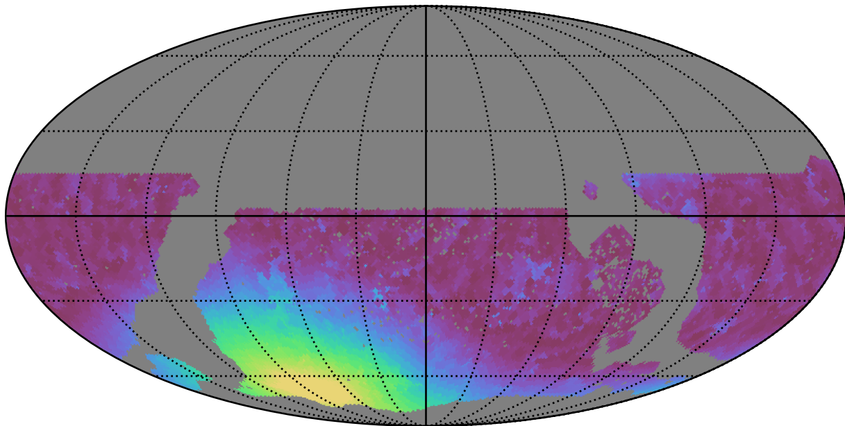
too_5_1v3.4_10yrs WFD r band: Min moonDistance
