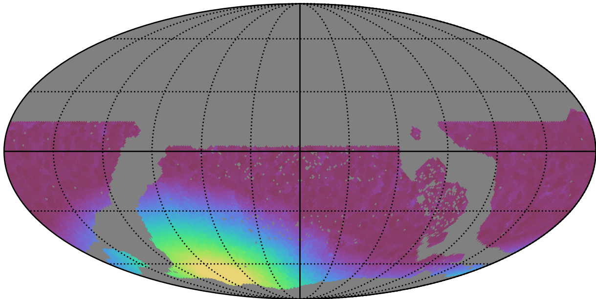
too_5_1v3.4_10yrs WFD i band: Min moonDistance
