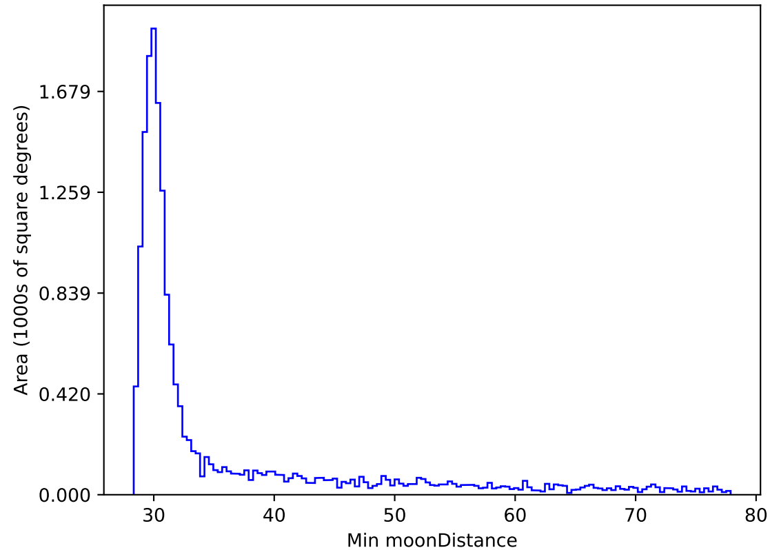
too_5_1v3.4_10yrs WFD i band: Min moonDistance
