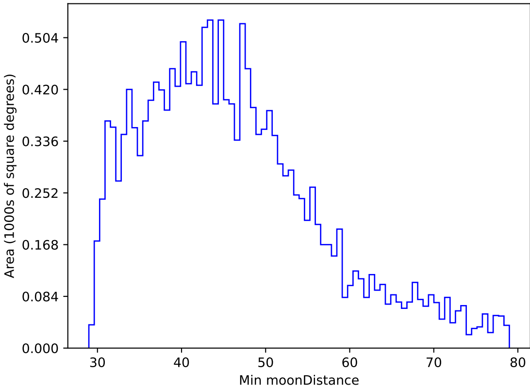
too_5_1v3.4_10yrs WFD g band: Min moonDistance
