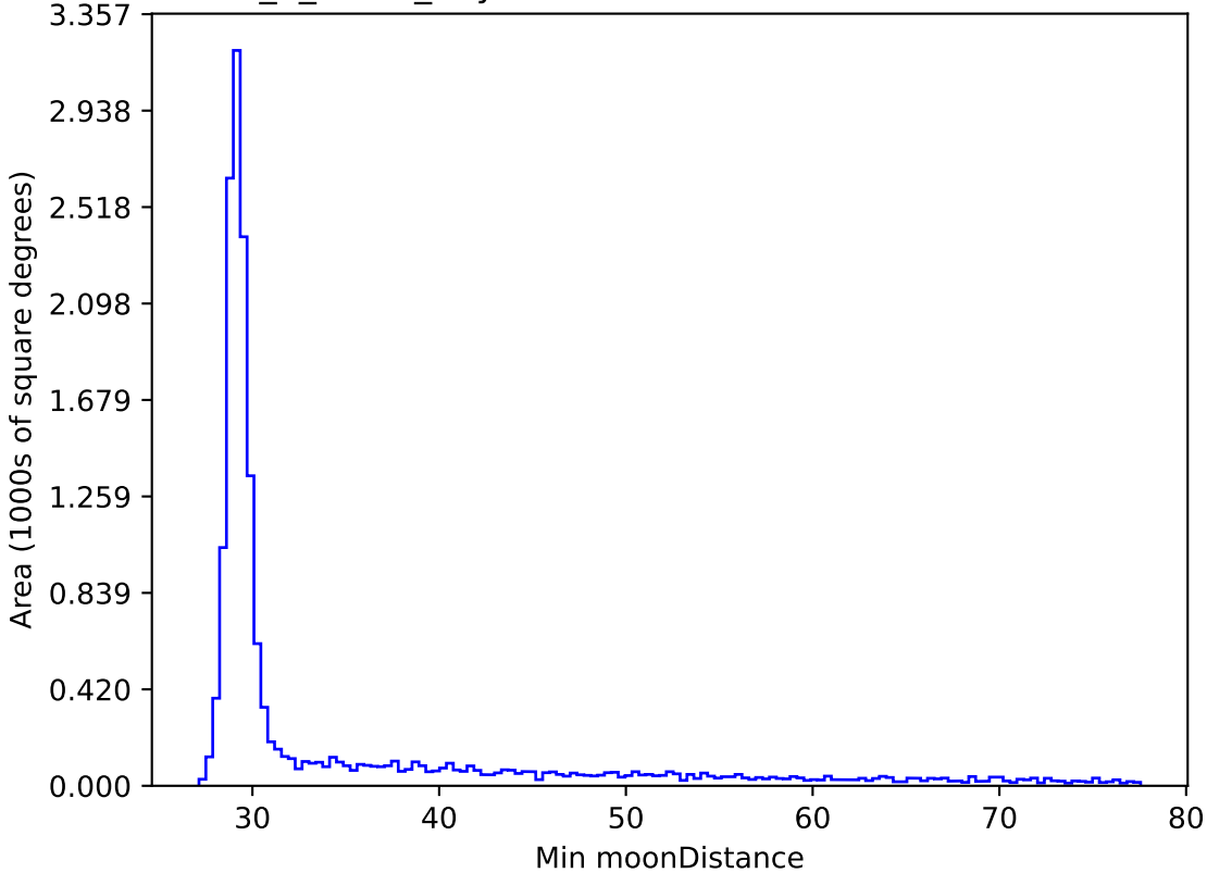
too_5_1v3.4_10yrs WFD all bands: Min moonDistance
