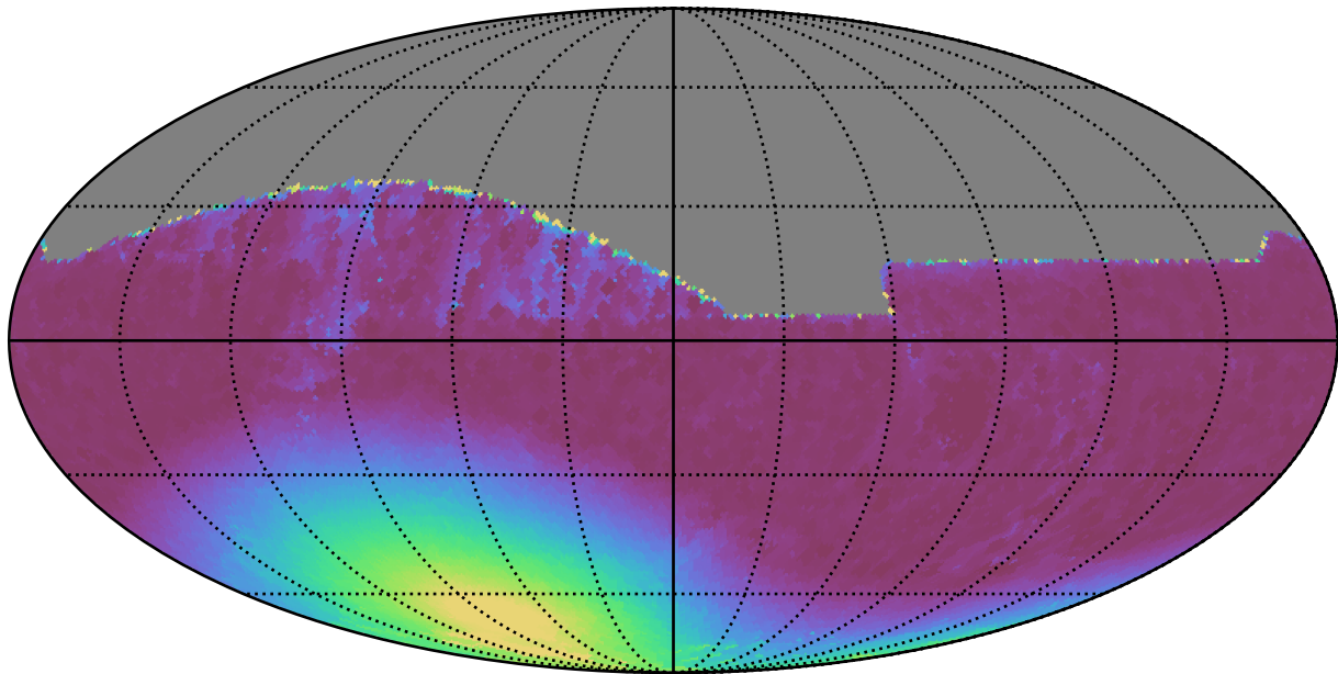
too_5_1v3.4_10yrs All sky z band: Min moonDistance
