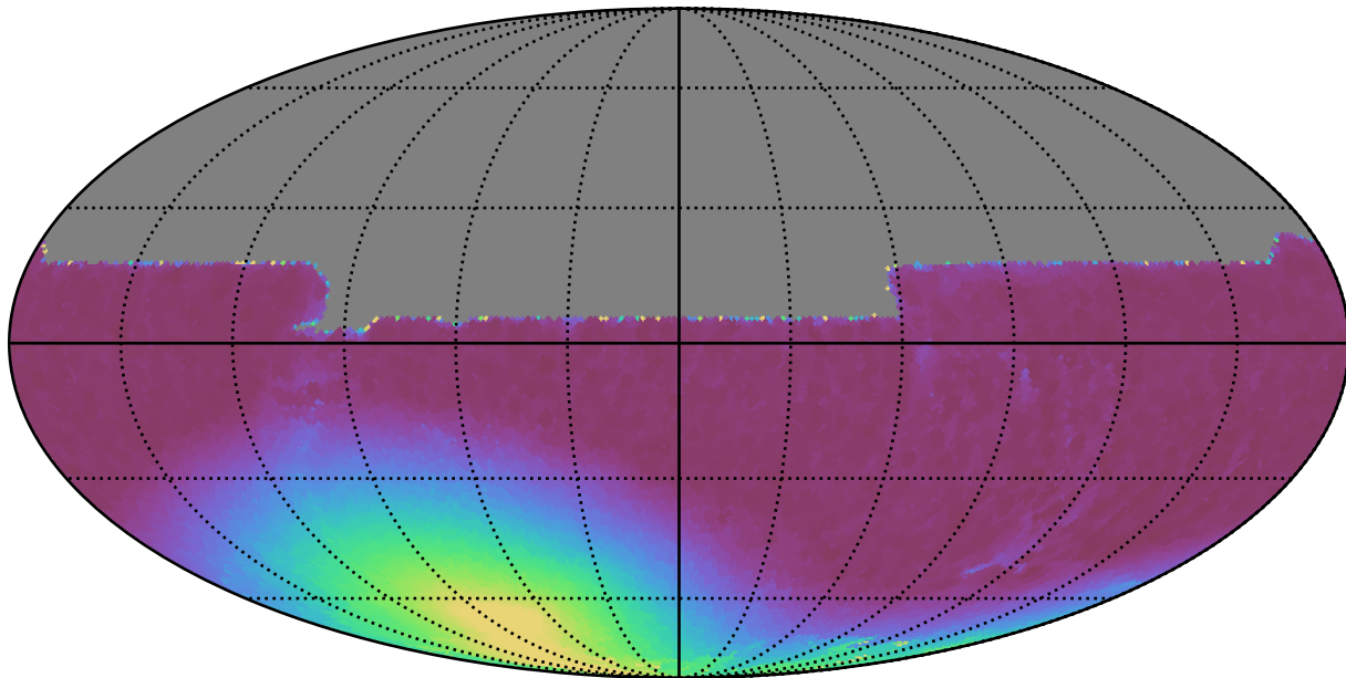
too_5_1v3.4_10yrs All sky y band: Min moonDistance
