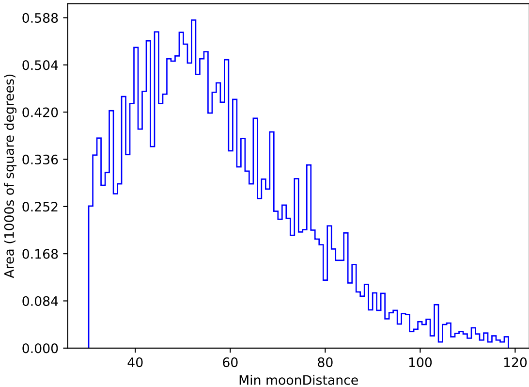
too_5_1v3.4_10yrs All sky u band: Min moonDistance
