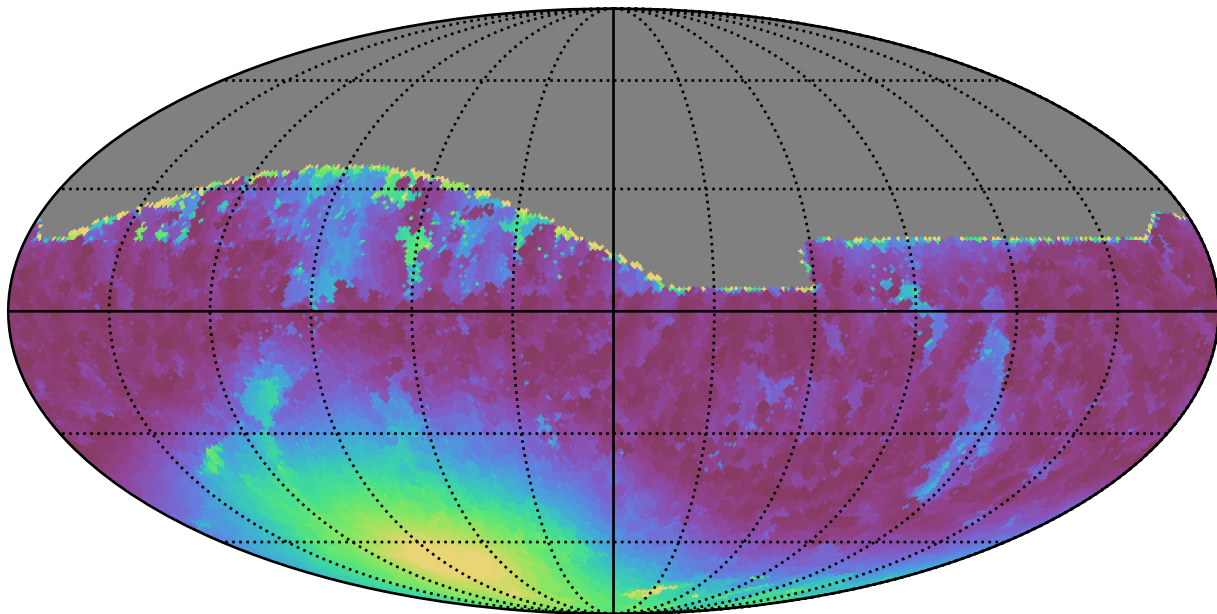
too_5_1v3.4_10yrs All sky r band: Min moonDistance
