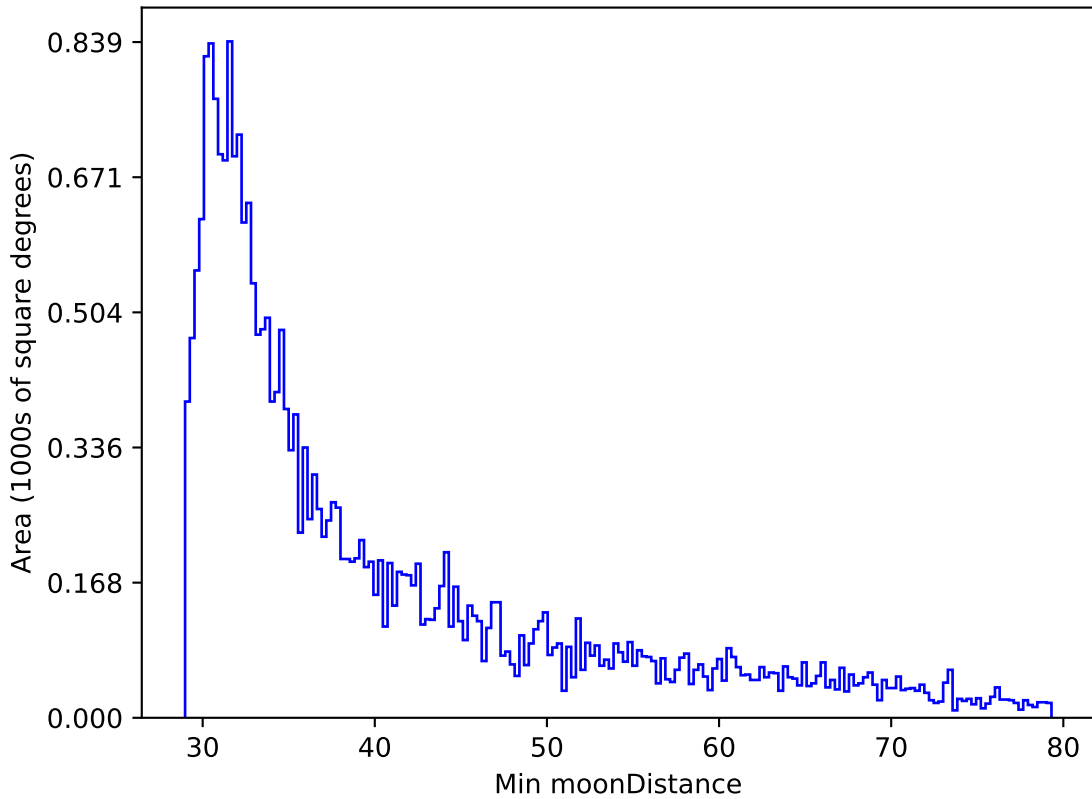
too_5_1v3.4_10yrs All sky r band: Min moonDistance
