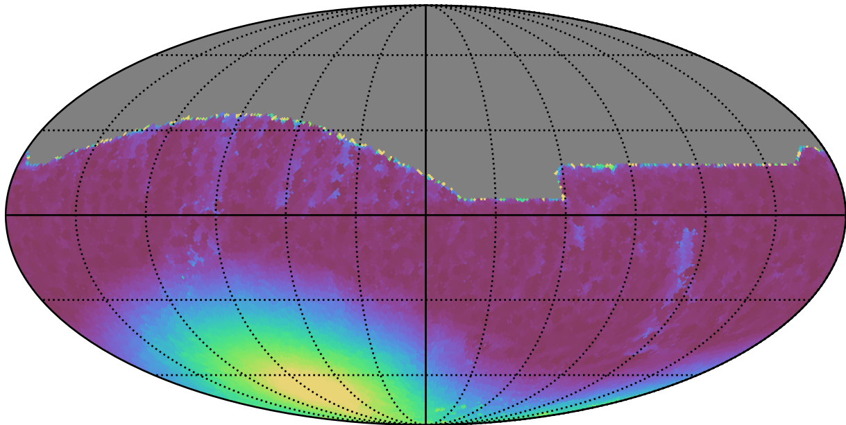
too_5_1v3.4_10yrs All sky i band: Min moonDistance
