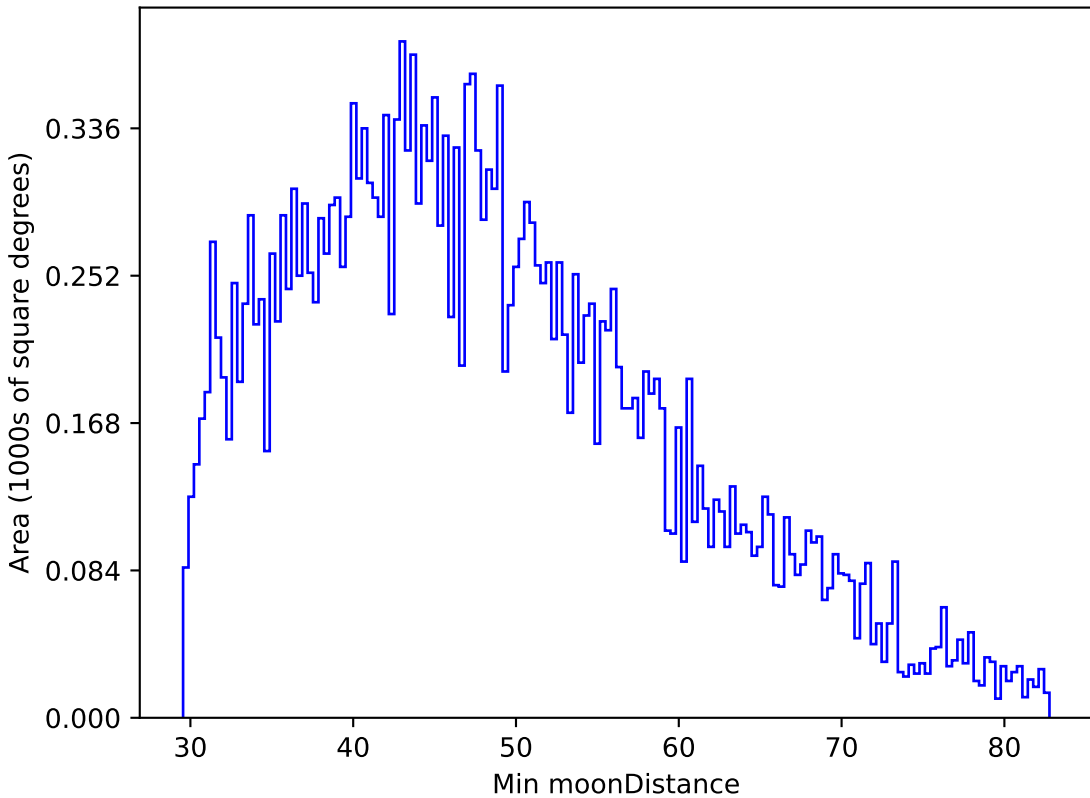
too_5_1v3.4_10yrs All sky g band: Min moonDistance
