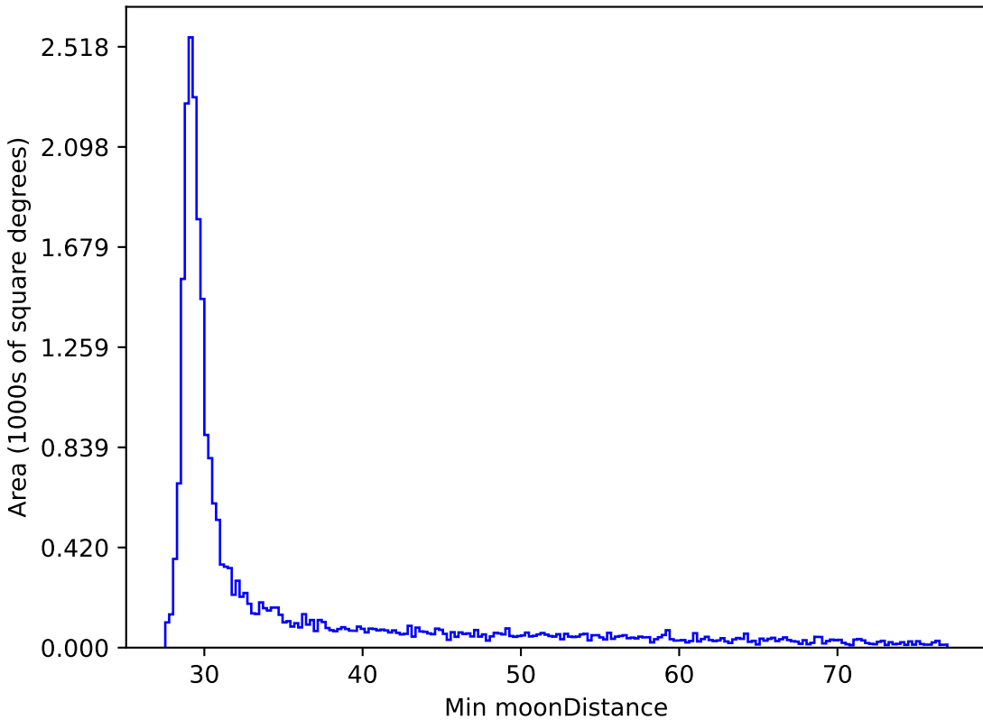
too_5_1v3.4_10yrs All sky all bands: Min moonDistance
