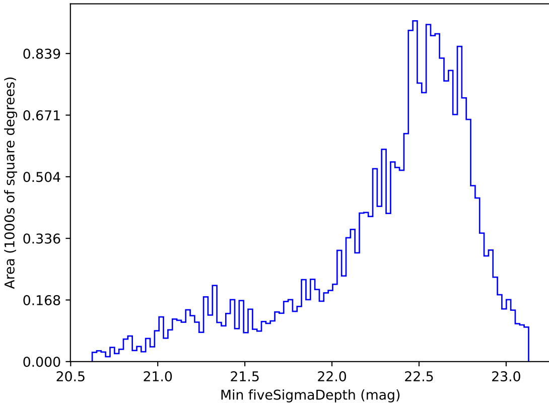
too_5_1v3.4_10yrs Yr 1 z band: Min fiveSigmaDepth
