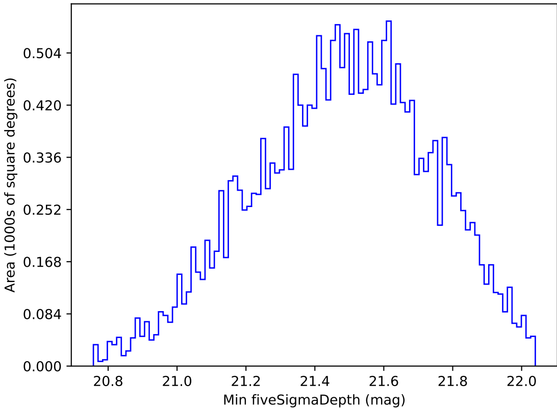
too_5_1v3.4_10yrs Yr 1 y band: Min fiveSigmaDepth
