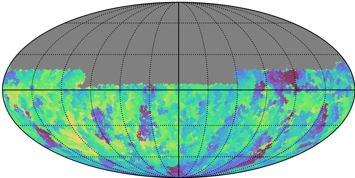
too_5_1v3.4_10yrs Yr 1 u band: Min fiveSigmaDepth
