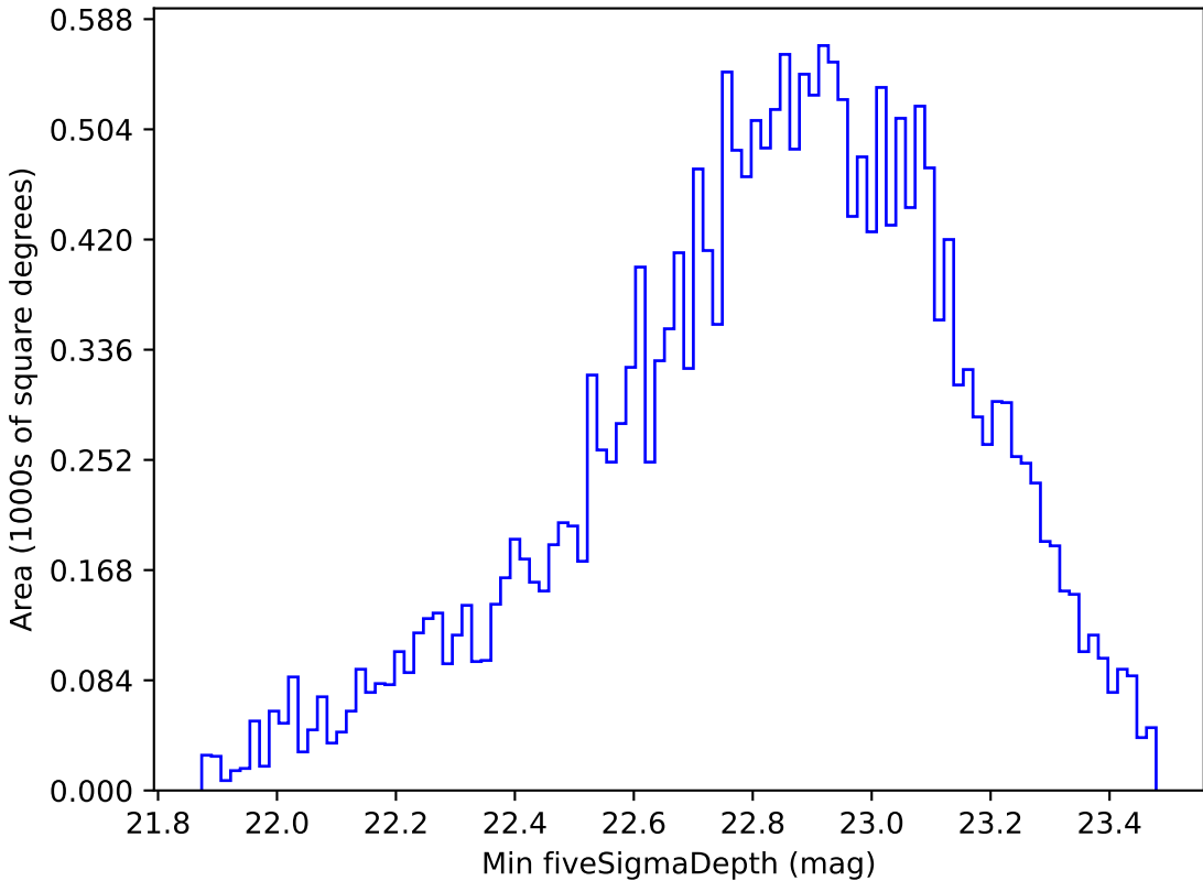
too_5_1v3.4_10yrs Yr 1 u band: Min fiveSigmaDepth
