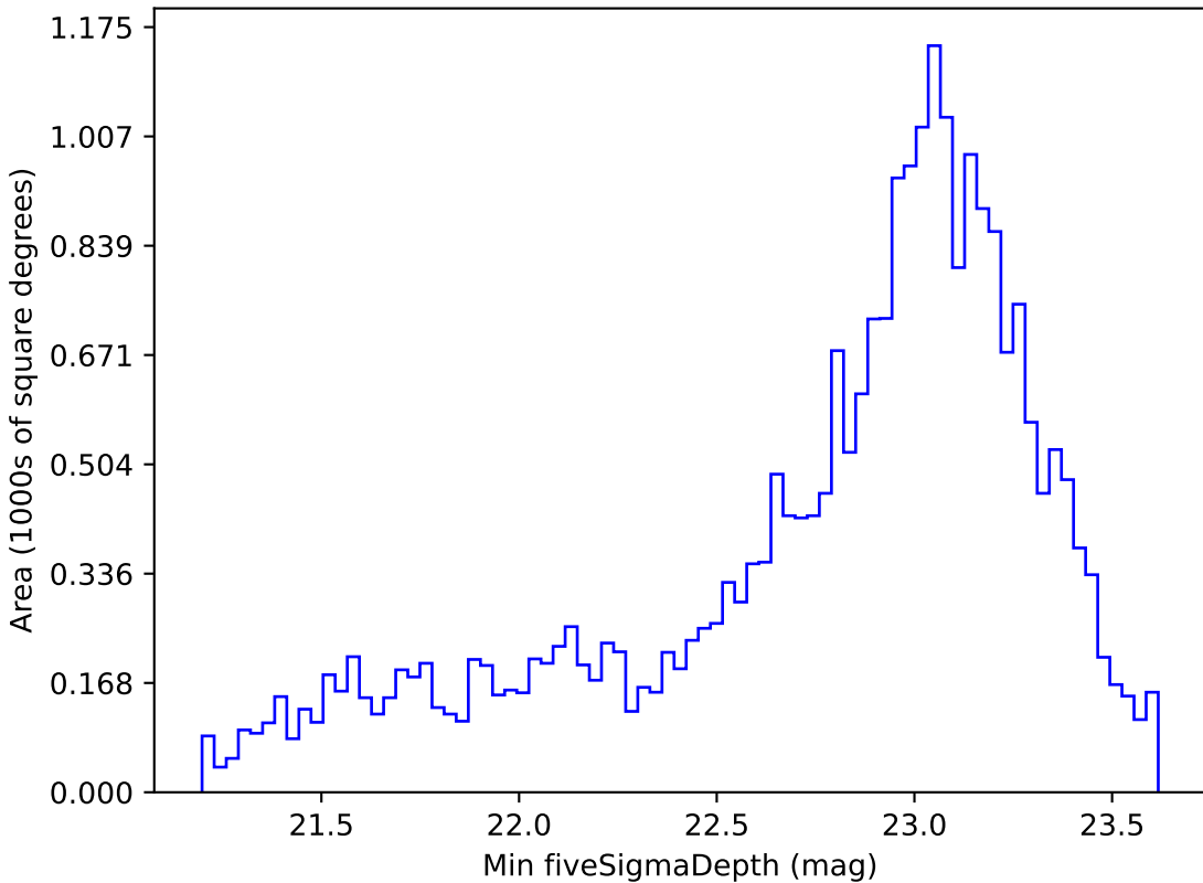
too_5_1v3.4_10yrs Yr 1 i band: Min fiveSigmaDepth
