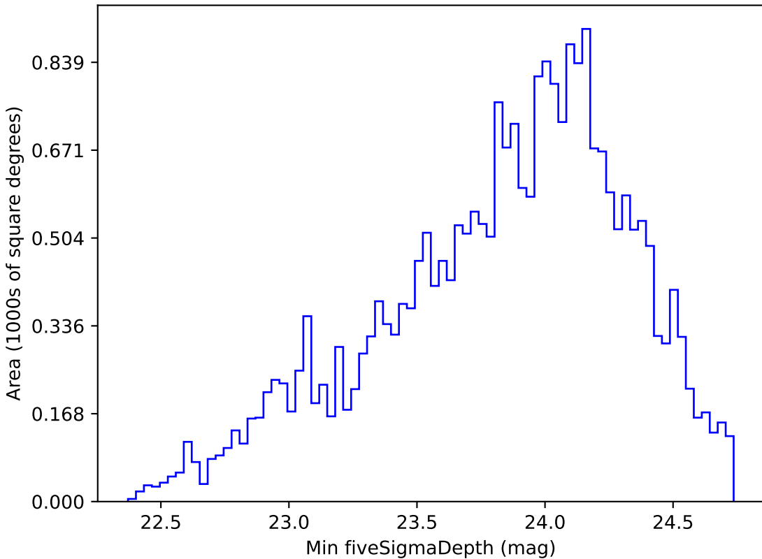
too_5_1v3.4_10yrs Yr 1 g band: Min fiveSigmaDepth
