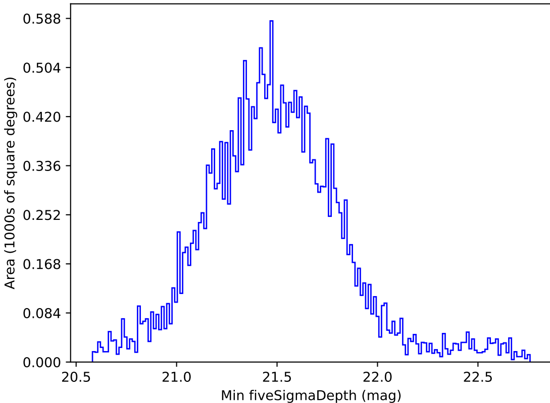
too_5_1v3.4_10yrs Yr 1 all bands: Min fiveSigmaDepth
