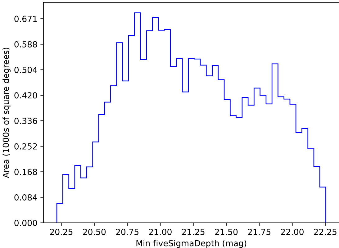
too_5_1v3.4_10yrs WFD z band: Min fiveSigmaDepth
