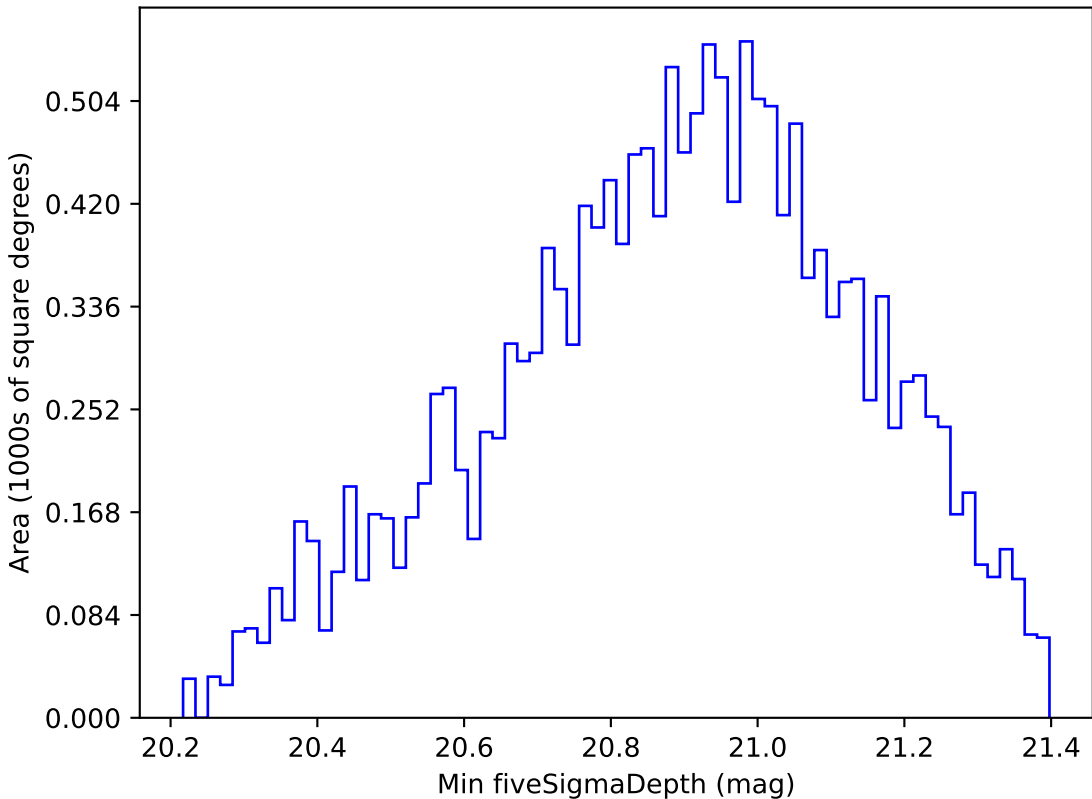
too_5_1v3.4_10yrs WFD y band: Min fiveSigmaDepth
