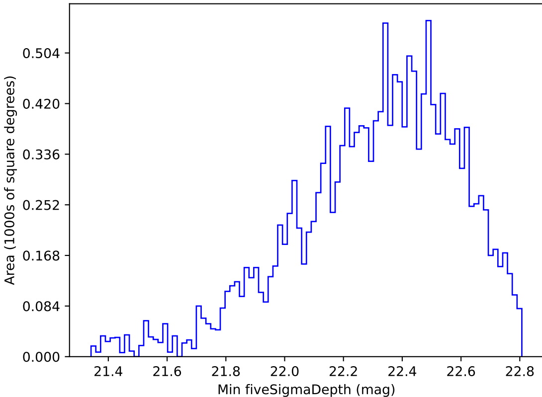
too_5_1v3.4_10yrs WFD u band: Min fiveSigmaDepth
