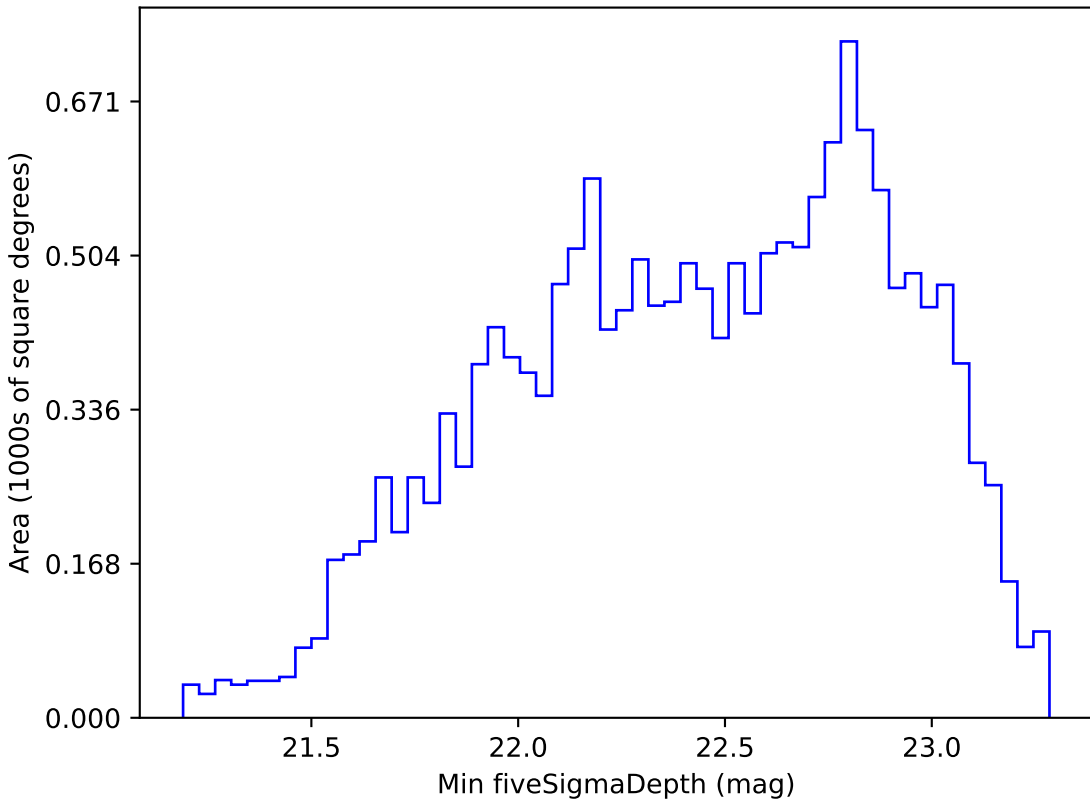
too_5_1v3.4_10yrs WFD r band: Min fiveSigmaDepth
