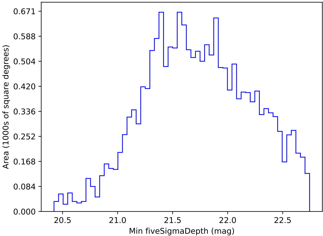
too_5_1v3.4_10yrs WFD i band: Min fiveSigmaDepth
