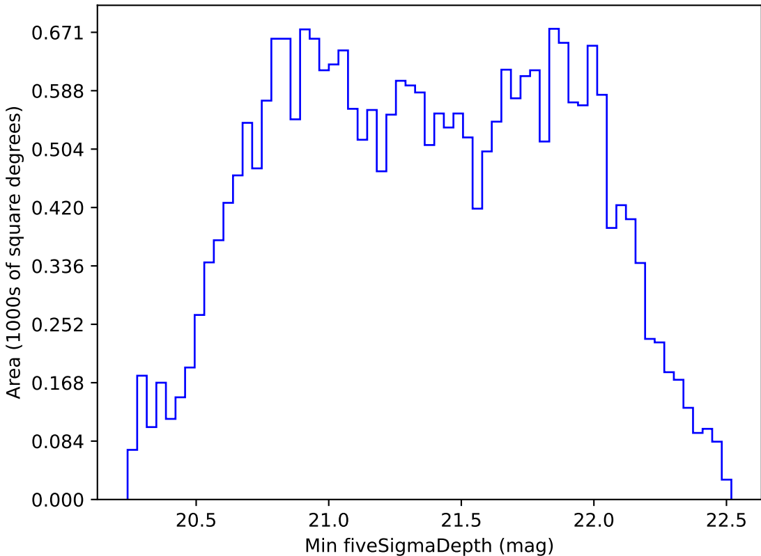
too_5_1v3.4_10yrs All sky z band: Min fiveSigmaDepth
