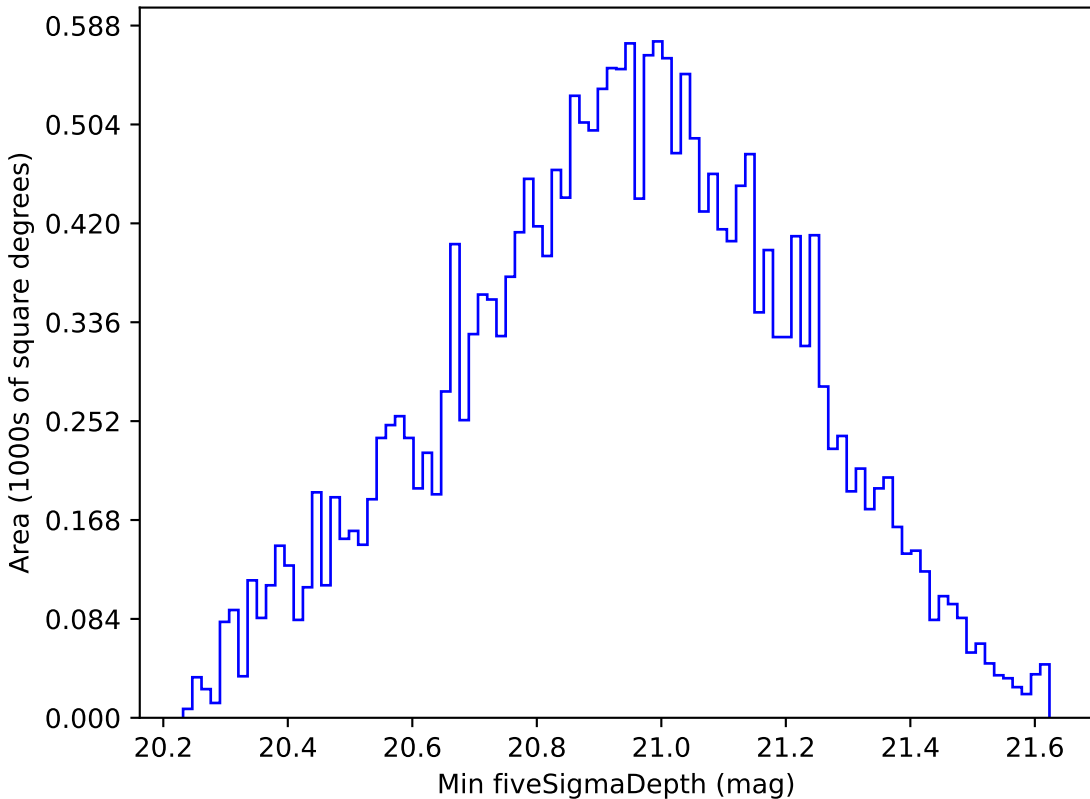
too_5_1v3.4_10yrs All sky y band: Min fiveSigmaDepth
